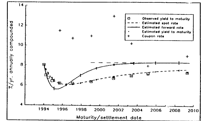
FIGURE A1A. Minimized Price Errors, Original N&S. Yields to Maturity, Spot and Forward Rates, Sweden, 29 December 1993 95 % confidence interval
