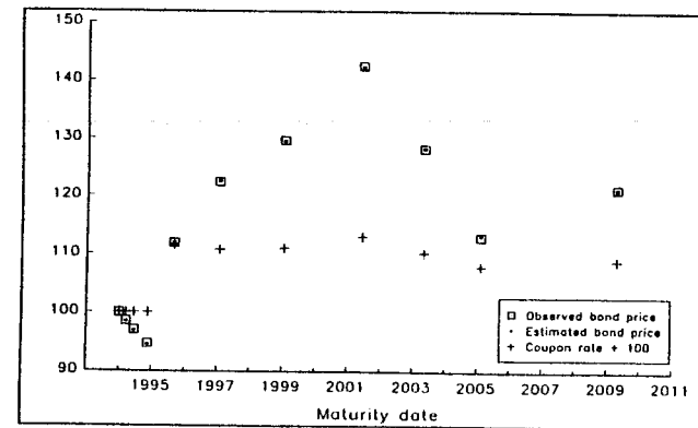
FIGURE A1B. Minimized Price Errors, Original N&S. Observed and Estimated Bond Prices, Coupons, Sweden, 29 December 1993 95 % confidence interval
