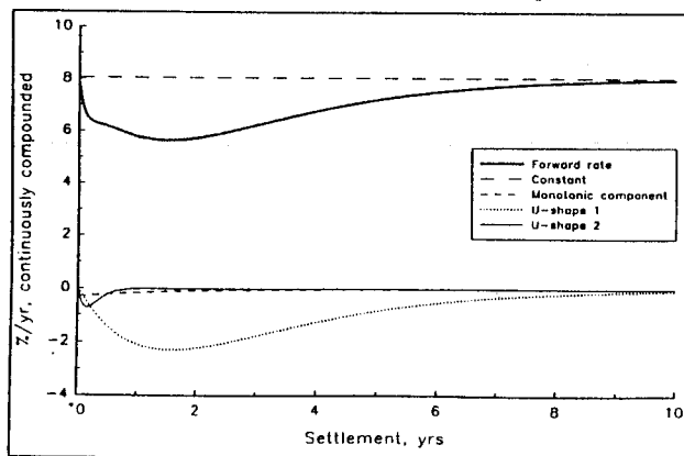
FIGURE 1. Forward Rate Curve and Components
