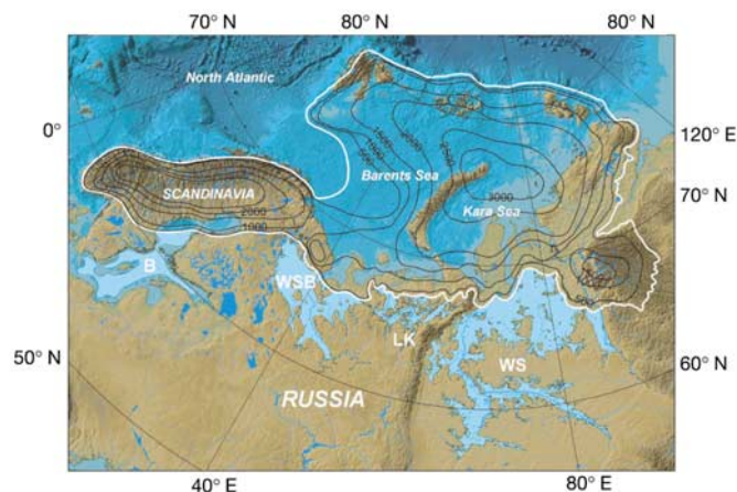
Figure 1 Maximum ice sheet and lake extent in northern Russia during the early Weichselian, about 90,000 yr ago. Abbreviations denote the West Siberian Lake (WS), Lake Komi (LK), the White Sea Basin Lake (WSB), and the Baltic Lake (B).
