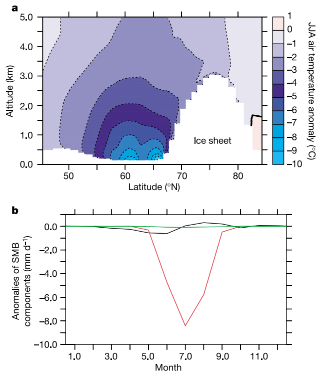
Figure 2 Lake-induced climate anomalies between simulation L and simulation NL. a , JJA (June, July, August) air temperature anomalies: vertical cut through the lower atmosphere at 70° E. The pattern is representative for all longitudes where proglacial lakes are adjacent to the Barents–Kara ice sheet. b , Monthly mean anomalies of surface mass balance (SMB) components precipitation (black), runoff (red) and evaporation/sublimation (green) on the Scandinavian/Barents–Kara ice sheet grid points that belong to the lakes' drainage basin.
