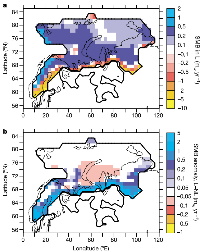
Figure 3 Simulated ice sheet surface mass balance and lake-induced surface mass balance anomaly. a , Simulated surface mass balance in simulation L; b , lake-induced surface mass balance anomaly (L–NL). Units are metres of water equivalent per year. Bold lines, ice sheets and lakes (grid-scale fraction > 20\% ) for 90 kyr ago; thin line, present-day coastline.
