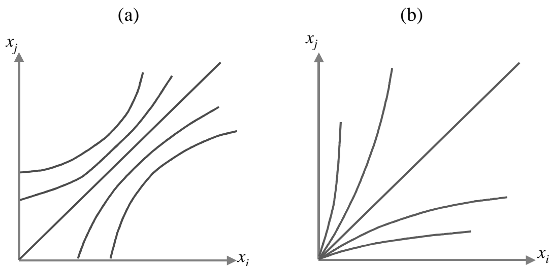
Figure 16: Inequality maps: (a) a variety of transformation directions; (b) the Dalton conjecture
